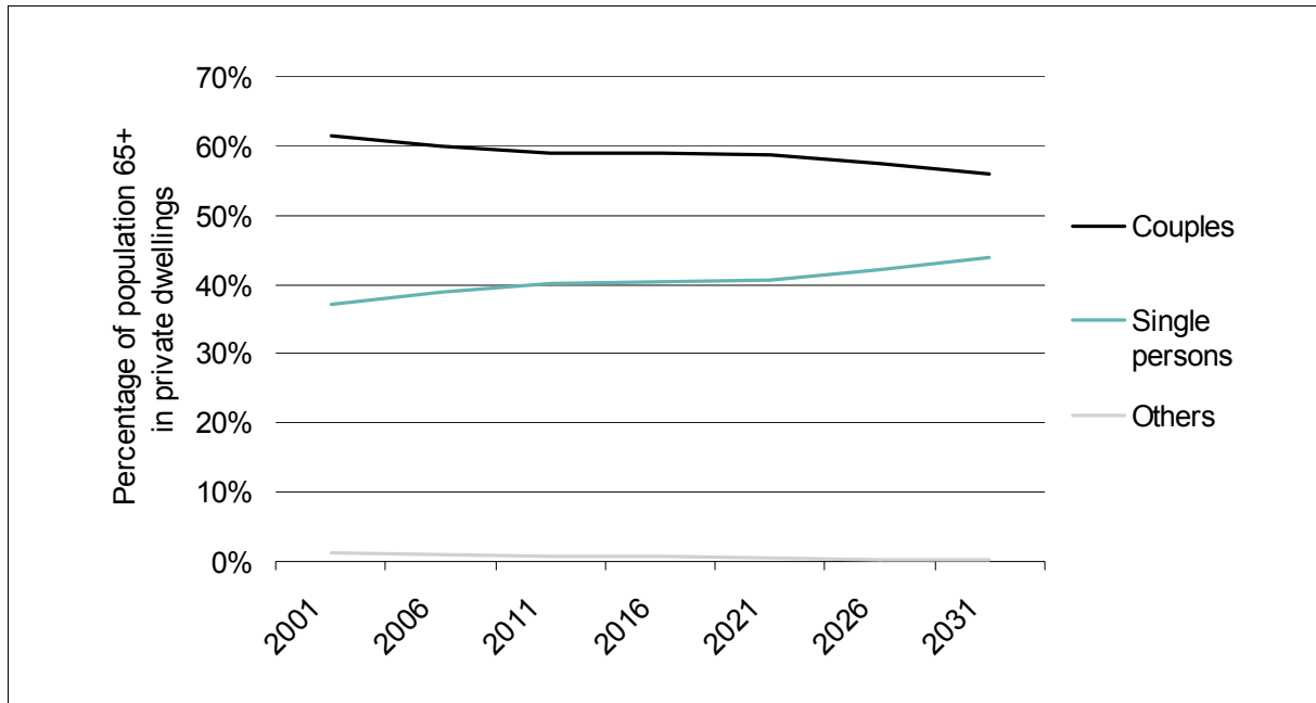
Figure 12 Projected changes in living arrangements of persons 65 years and older, Australia 2001-2031
