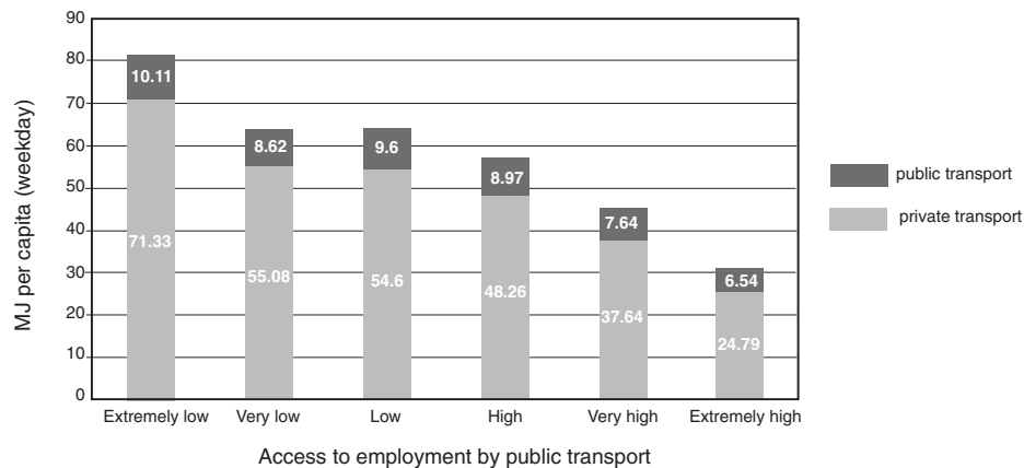
Figure 2 Energy consumption intensity by mode in Sydney
