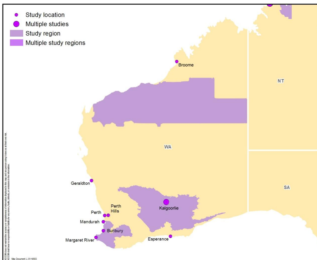
Figure ES1: Case study locations of synthesised adaptation research in Western Australia
