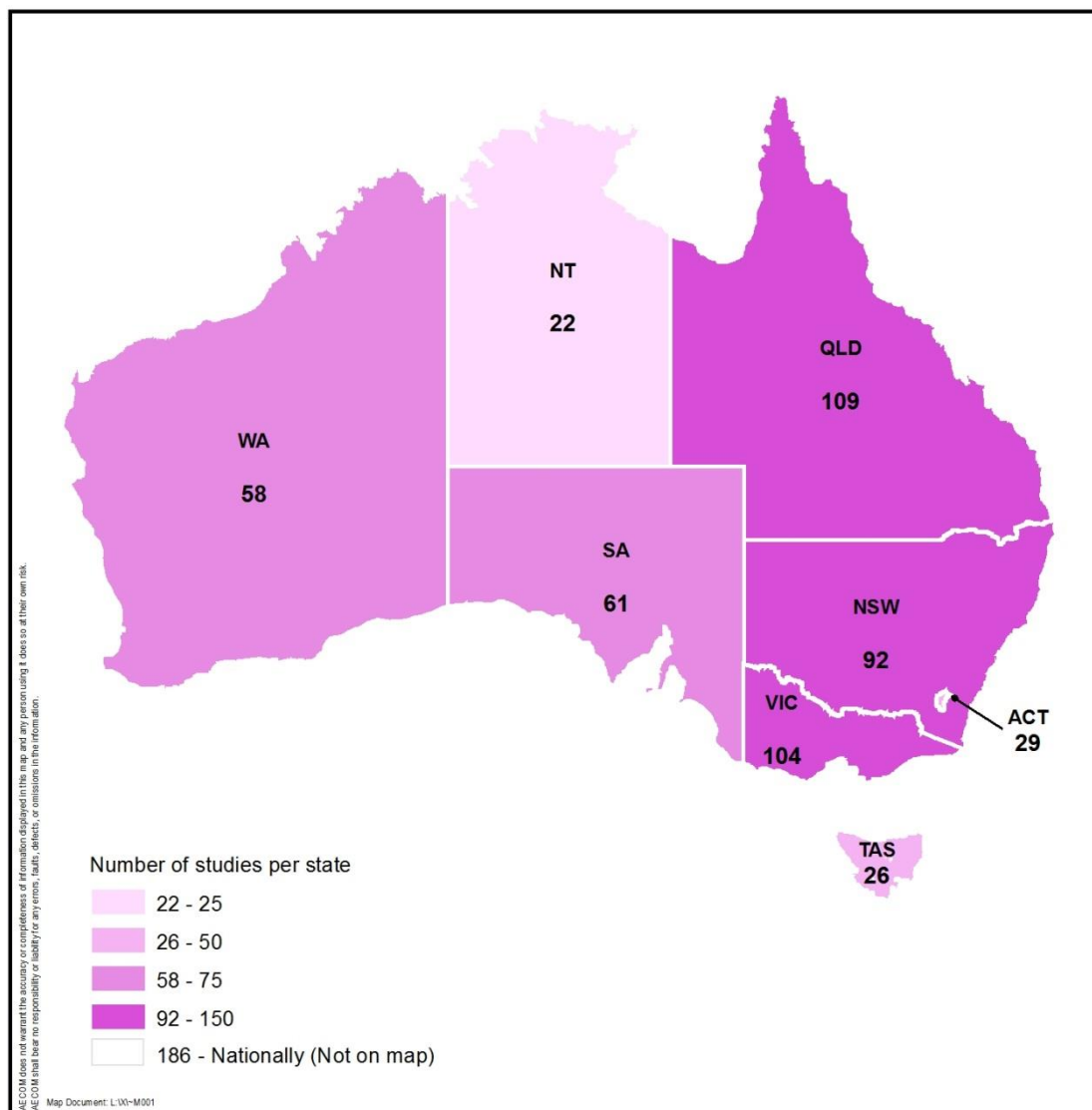
Figure 2: NCCARF and non-NCCARF research by state/territory
