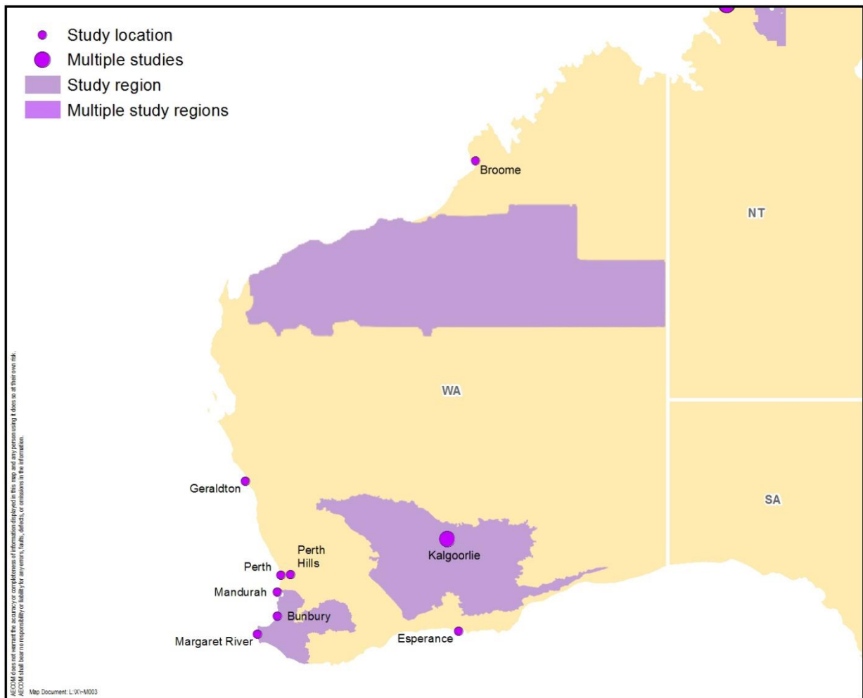
Figure 3: Case study locations of identified adaptation research in Western Australia
