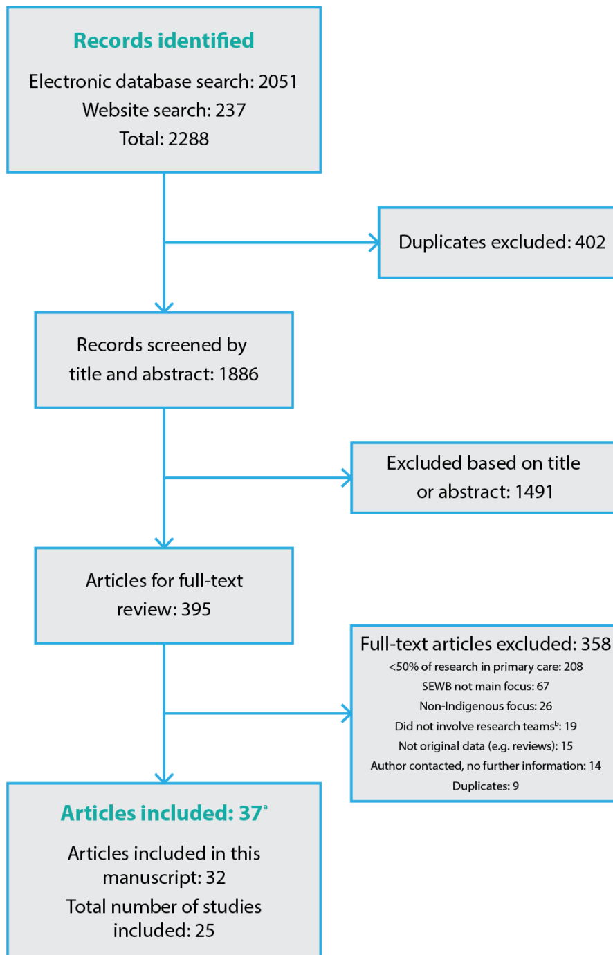
Figure 1. PRISMA diagram of the systematic review process
