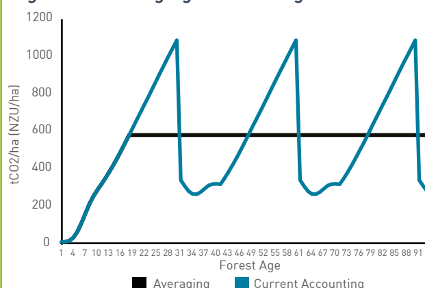
Figure 3: “Averaging” accounting
