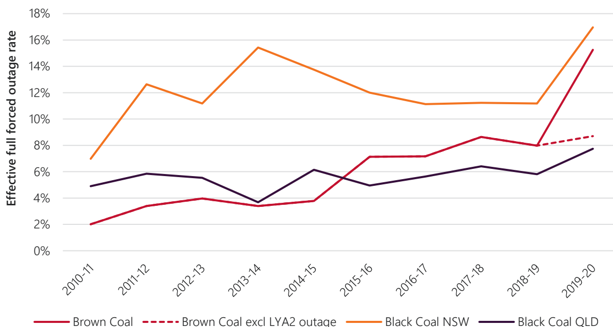
Figure 21 Historical outage rates for coal-fired generator technologies
