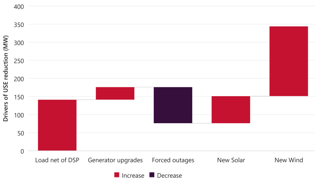
Figure 23 Drivers of expected USE reduction in Victoria (2020 ESOO forecast of 2020-21 vs 2019 ESOO forecast of 2019-20) – excluding Loy Yang A/Mortlake outage impact
