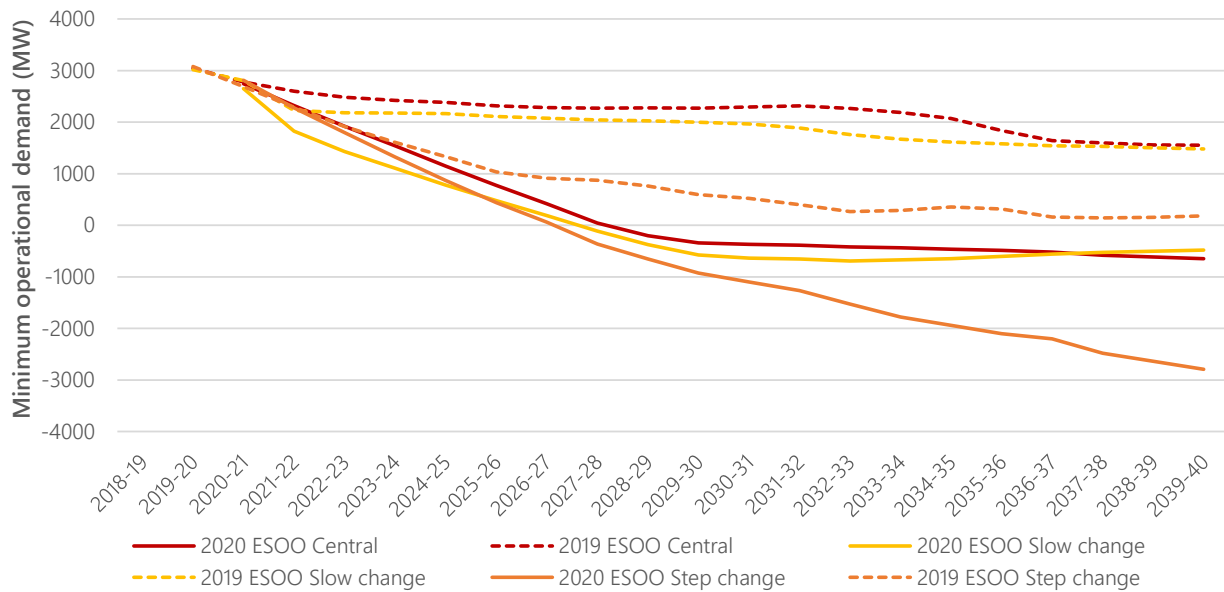
Figure 18 Forecast shoulder 50% POE minimum operational demand (sent out) by scenario, Victoria
