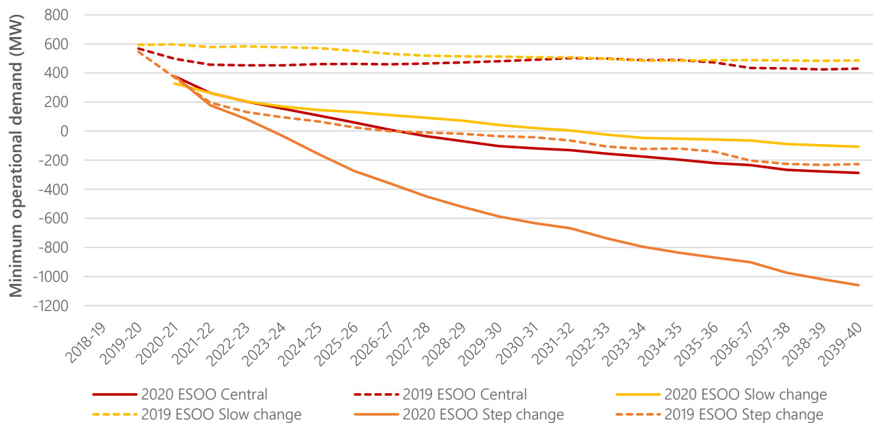
Figure 17 Forecast shoulder 50% POE minimum operational demand (sent out) by scenario, South Australia
