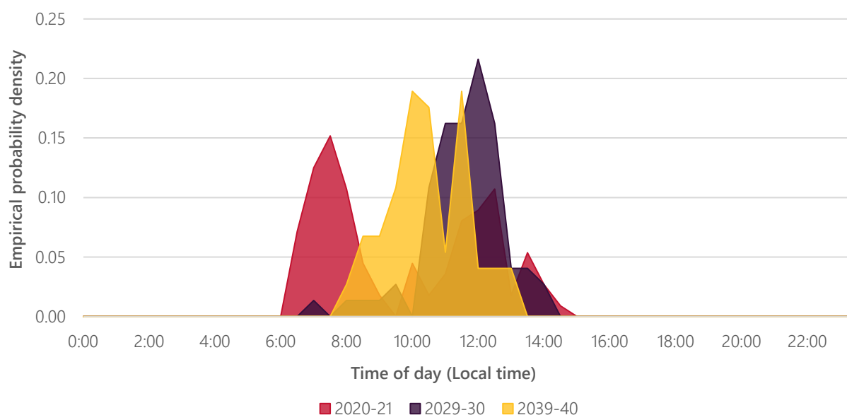
Figure 46 Distribution of forecast time of 50% POE shoulder minimum demand in New South Wales
