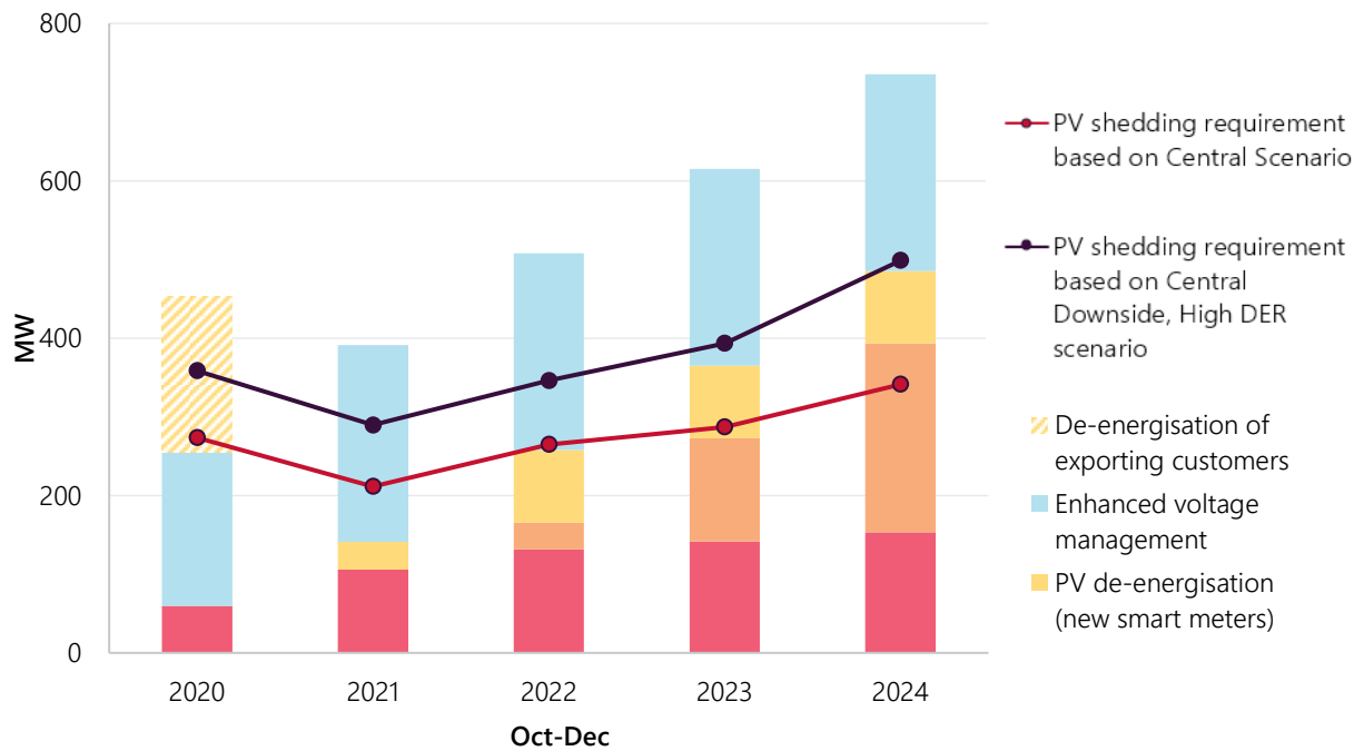
Figure 71 Emergency PV shedding capacity required in South Australia with identified options (90% POE minimum demand)
