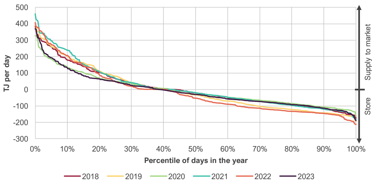
Figure 33 Cumulative distribution of net changes in storage level for Iona UGS, 1 January 2018 to 31 December 2023 (TJ/d)
