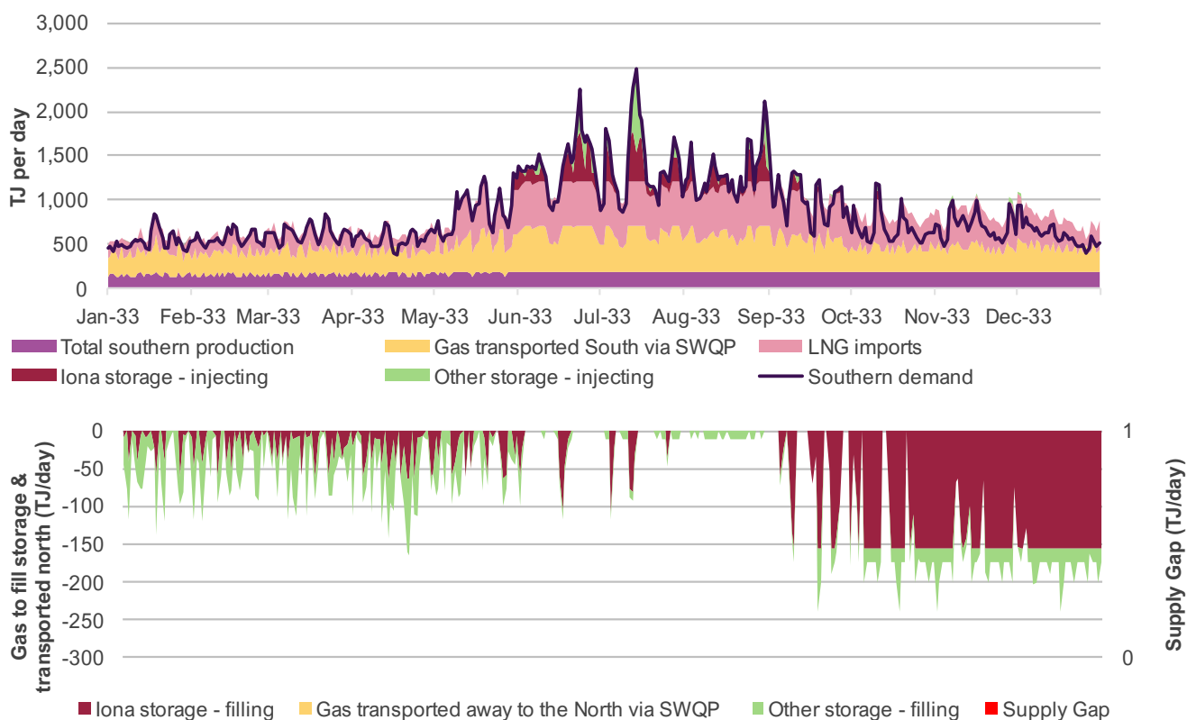
Figure 53 Supply-demand balance for the LNG import terminal option, 2033, Step Change (TJ/d)
