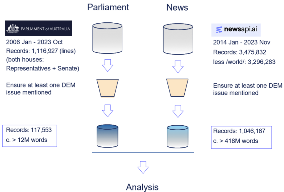
Figure 1: Data pipeline
