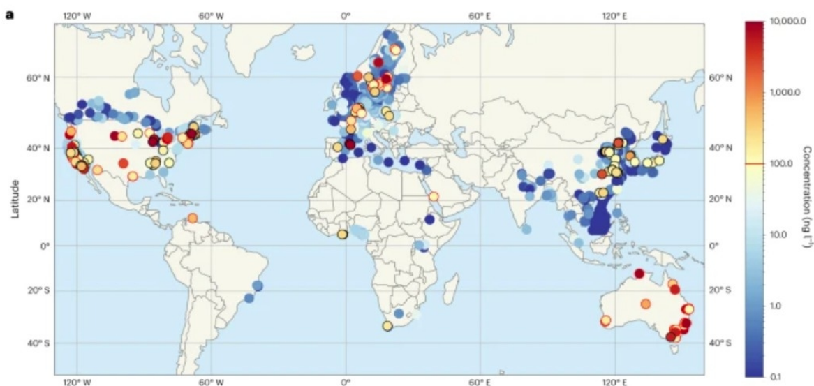
Figure 4.1 Global map of PFAS concentration in water (published 2024)
