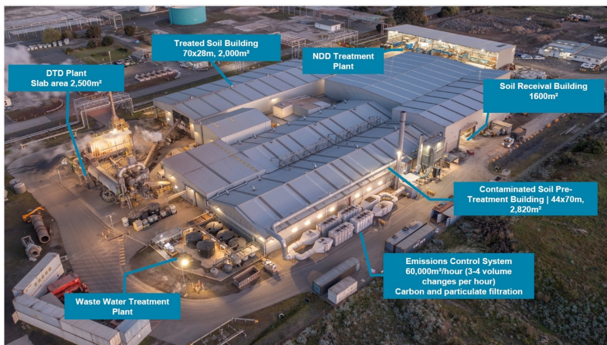
Figure 2.2 SOLVE thermal desorption plant, Altona, VIC
